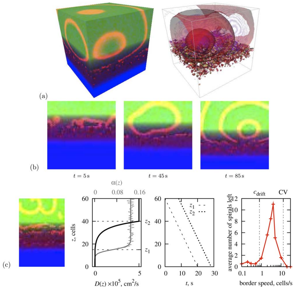
Figure 11. The ischaemic border zone in three dimensions. “Toy” set of parameters: D_{\max} = 5 \cdot 10^{-5} cm 2 /s, \alpha_{\max} = 0.13 , \delta_z = 0.1 . (a,b) Box size 60 \times 60 \times 60 cells, border speed c = 1/6 cell/s. (a) Snapshot of activity on the surface and inside the box (red semi-transparent surfaces are excitation fronts). (b) Activation patterns on a middle cross-section of the box. (c) Schematic of the study of spirals’ probability to escape to the well-coupled zone: a snapshot through the middle of a thin 3D layer of cells (box size 40 \times 5 \times 60 , border speed c = 3 cell/s); corresponding distribution of D , \bar{\alpha} and z ; movement of boundaries with time; and average number of spirals left in the box after passing of the border zone, as function of the its speed. Here c_{\text{drift}} is a typical drift velocity and CV is a typical conduction velocity. doi:10.1371/journal.pone.0024388.g011
